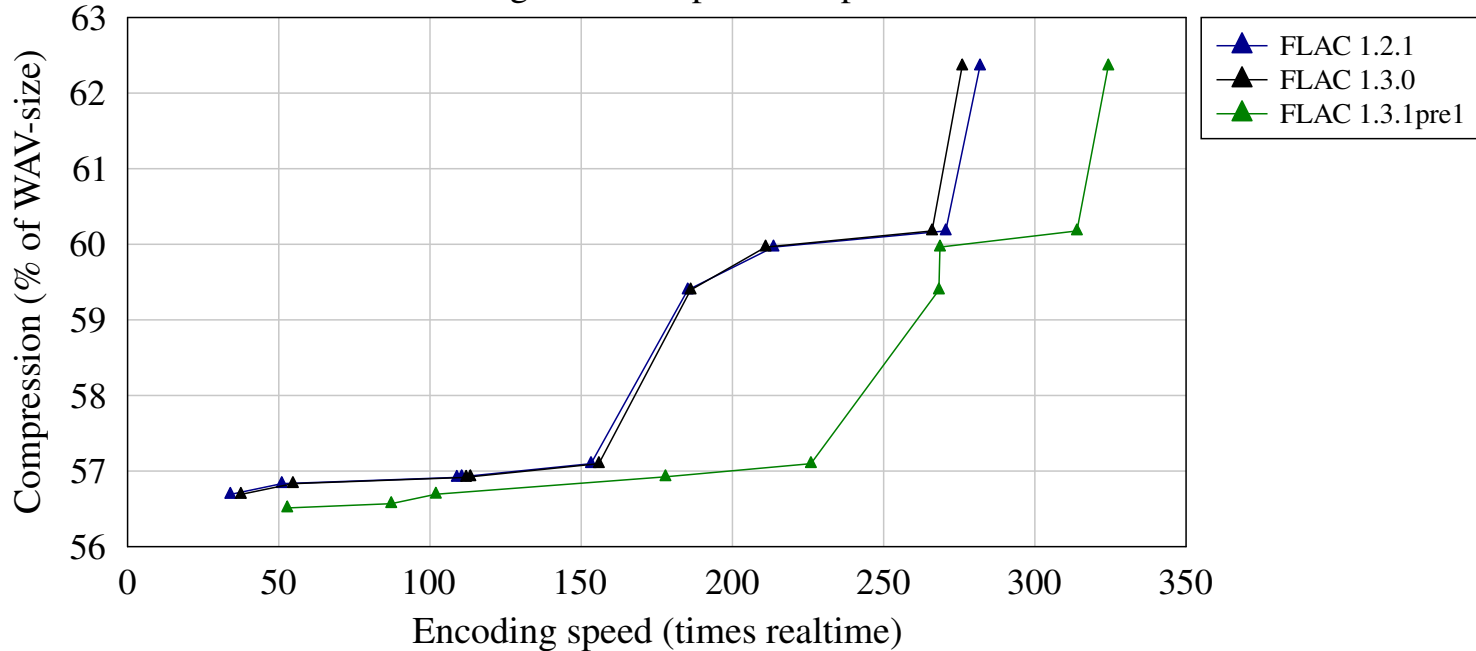
Encoding speed vs compression for long set of samples-1.3.1pre1
