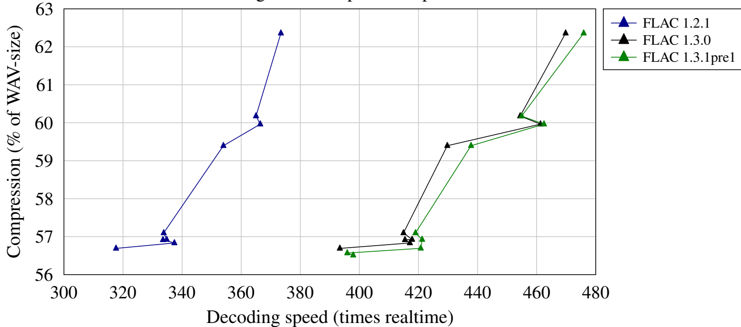
Decoding speed vs compression for long set of samples-1.3.1pre1
