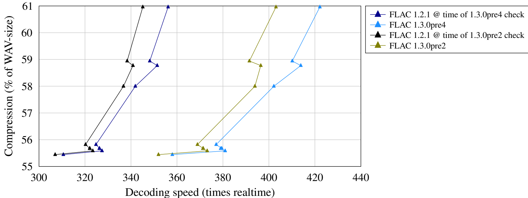
Decoding speed vs compression (All tracks)
